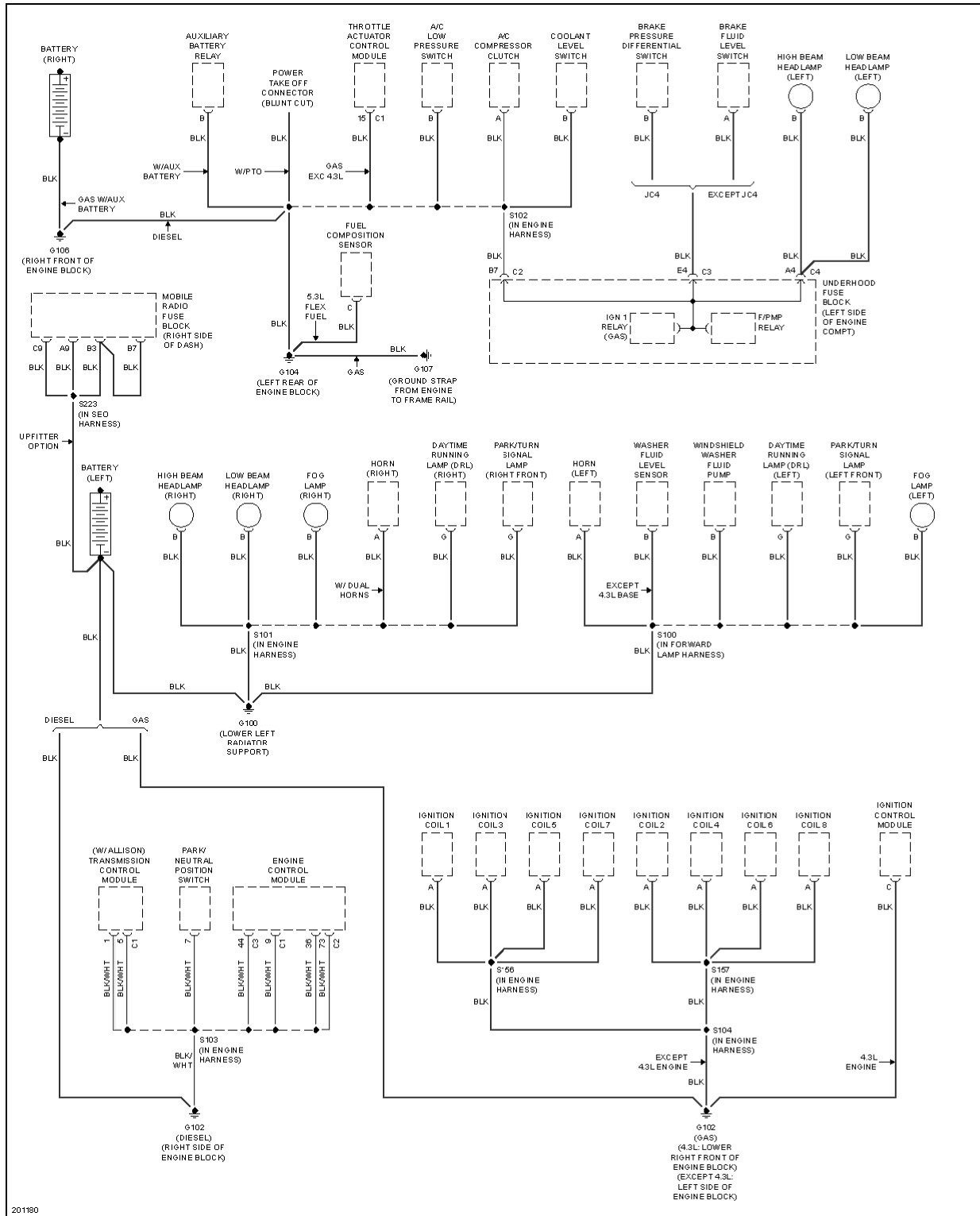
Fig. 57: Ground Distribution Circuit, Except Hybrid (1 of 4)
